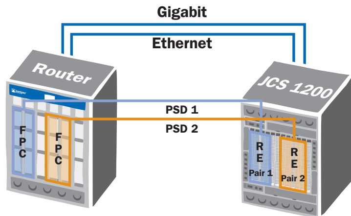
JCS 1200 Architecture
